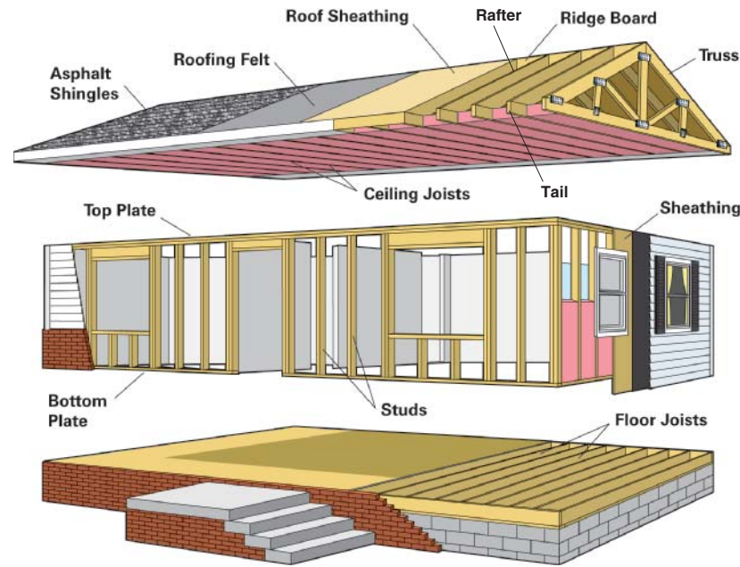
Figure 19.2 The House Structure with Gable Roof
