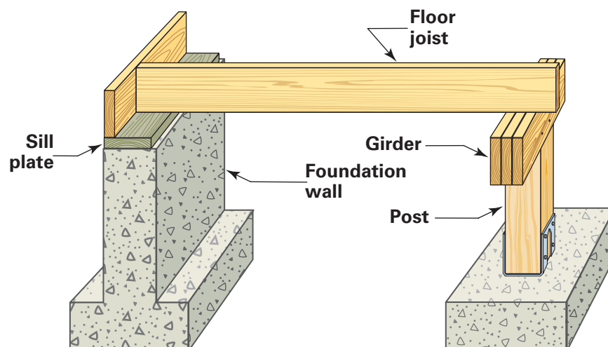
Figure 19.1 Floor Joists
