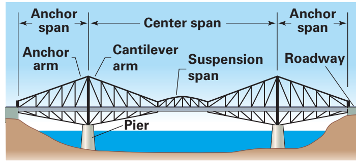
CANTILEVER BRIDGE
