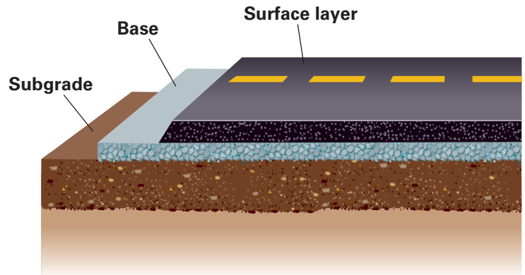
Figure 20.1 Paved Roads
